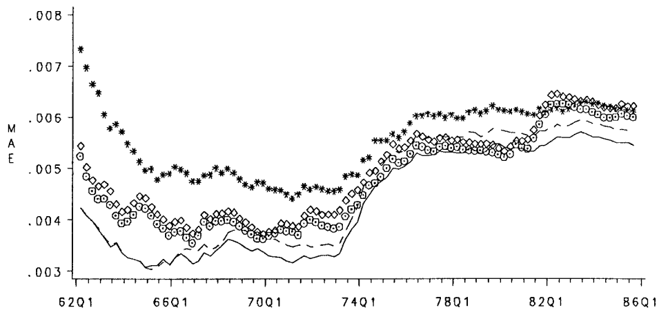
Fig. 16. Root Mean Squared and Mean Absolute Errors of the Two Quarter Ahead Inflation Forecasting Models. The symbols are: Random Walk (Star), Time Series (Line), Time Series Window (Dash), Treasury Bill-Average (Circle) and Treasury Bill-Spot (Diamond).
