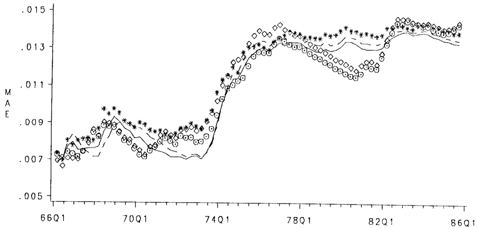
Fig. 18. Root Mean Squared and Mean Absolute Errors of the Four Quarter Ahead Inflation Forecasting Models. The symbols are: Random Walk (Star), Time Series (Line), Time Series Window (Dash), Treasury Bill-Average (Circle) and Treasury Bill-Spot (Diamond).
