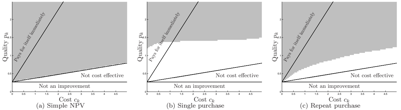
Figure 2: Adoption regions for the example of Figure 1
