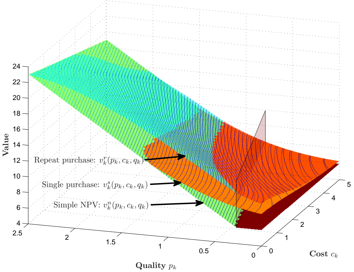
Figure 1: Value functions for the numerical example of §2.3 (with k=10 periods to go)
